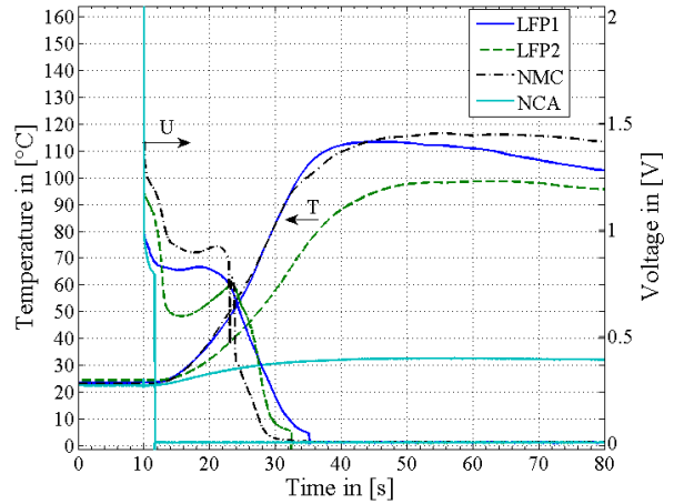
Figure 6: Temperature and voltage profiles for short circuit tests
