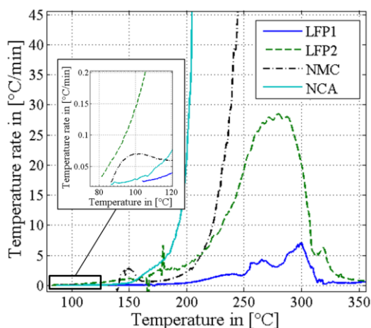
Figure 3: Results of the performed ARC tests with zoom at onset temperature of self-heating
