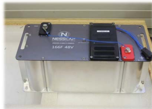
48V module (18 x 3000F cells)
